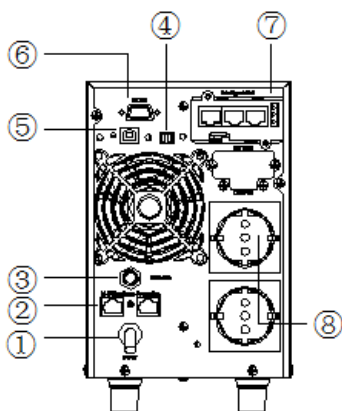
1 kVa (S):
