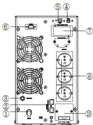
2/3 kVa (S):
